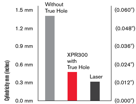
10 mm holes, 9.5 mm mild steel plate, 130 A process (0.394" holes, 3/8" mild steel plate)
